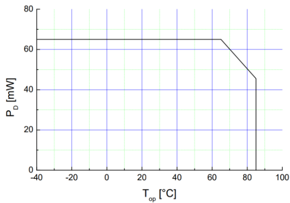
Maximum Ratings (1)
