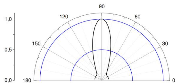
Radiation Pattern
