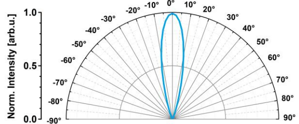
Radiation Pattern
