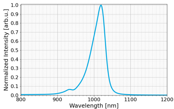
Optical Spectrum
