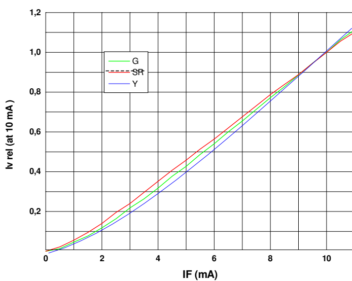
I_F - I_{v, \text{rel}} characteristic
