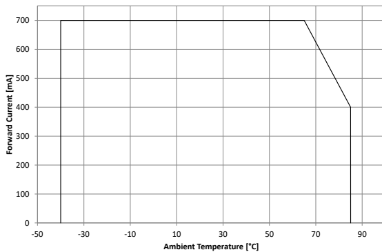
Maximum Ratings (1)
