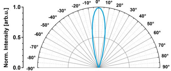
Radiation Pattern
