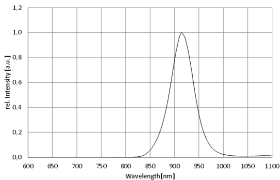
Optical Spectrum
