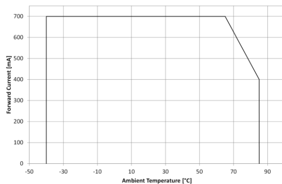
Maximum Ratings (1)
