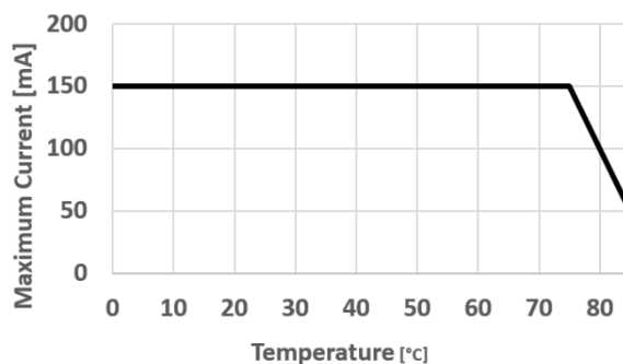
Maximum Ratings (1)
