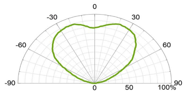
Radiation Pattern
