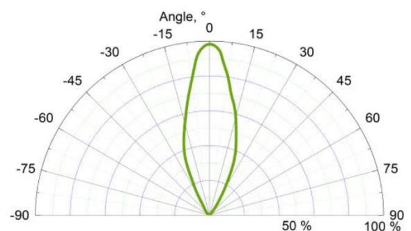
Radiation Pattern
