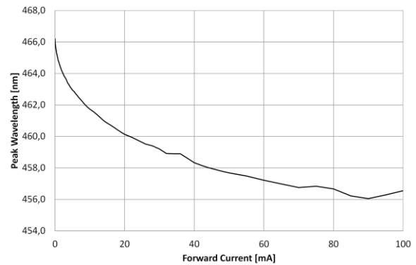
Wavelength Shift vs. Forward Current
