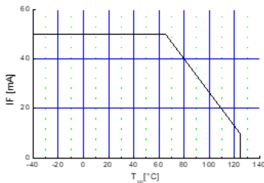
Maximum Ratings (1)
