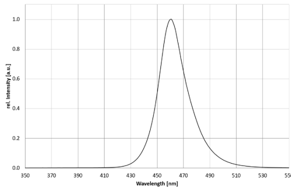
Optical Spectrum
