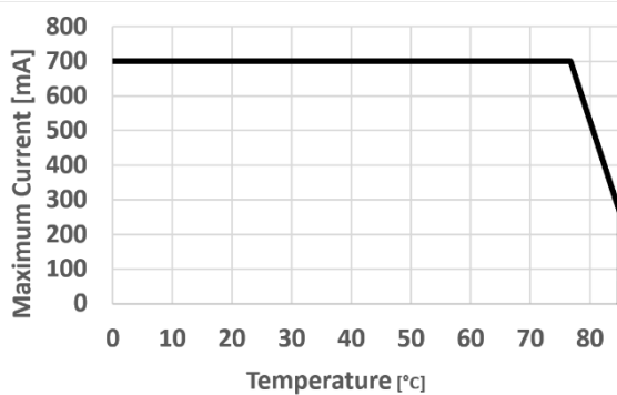
Maximum Ratings (1)
