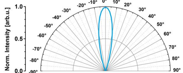
Radiation Pattern
