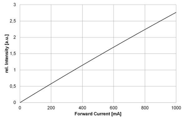
Relative Intensity vs. Forward Current
