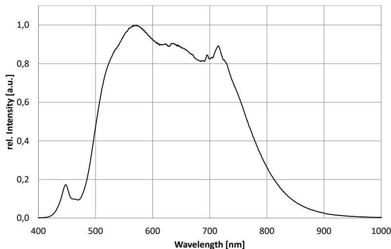
Relative Spectral Emission Spektrum
