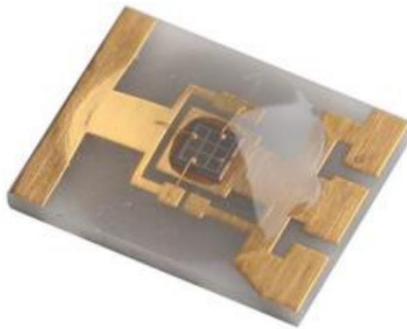
High Power Green LED with Glob Top
