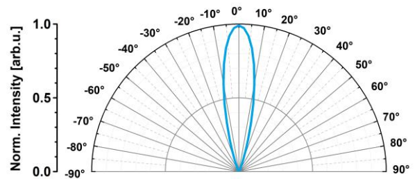
Radiation Pattern
