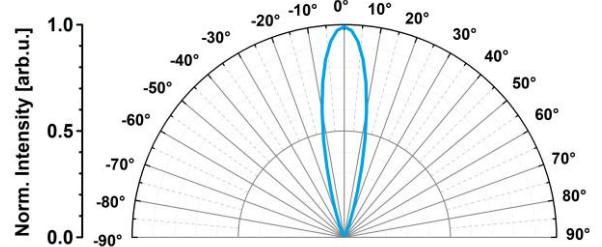
Radiation Pattern
