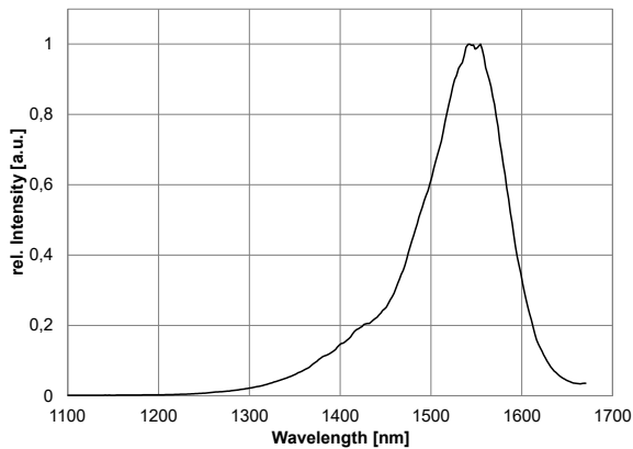
Optical Spectrum
