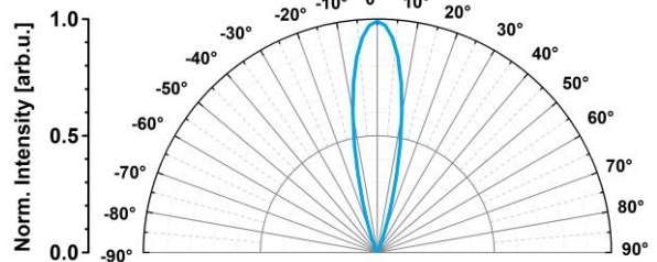
Radiation Pattern
