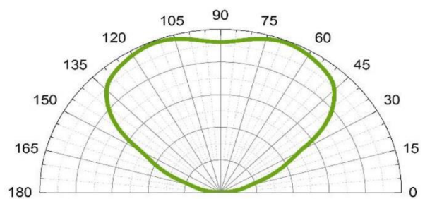
Radiation pattern Radiation Pattern
