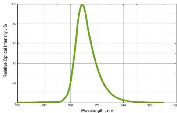
Optical Spectrum
