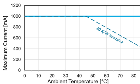
Maximum Ratings (1)
