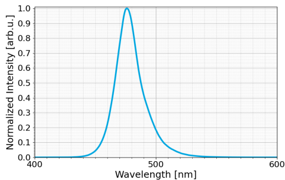
Optical Spectrum
