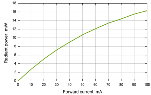
Radiant Power vs. Forward Current
