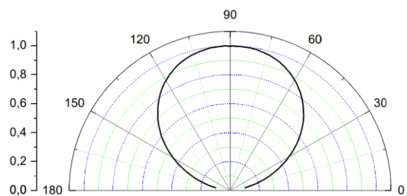
Radiation Pattern
