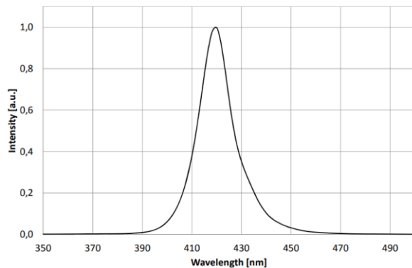
Optical Spectrum
