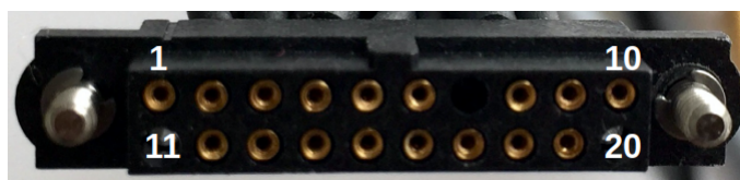
Figure 4.5: C-S2m-IN cable connector (female) to the S-2m input (male), Sec. 4.1.
