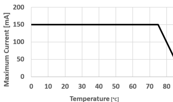
Maximum Ratings (1)
