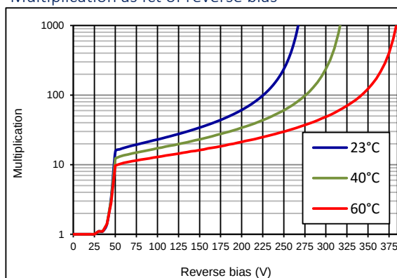
Multiplication as fct of reverse bias
