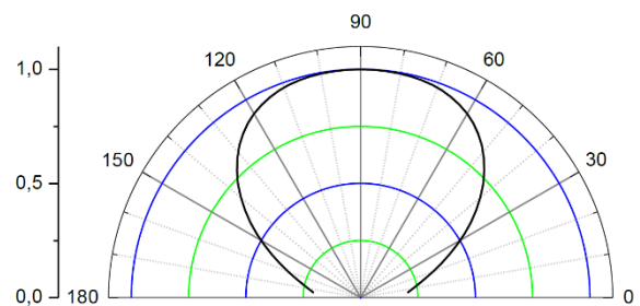
Radiation Pattern
