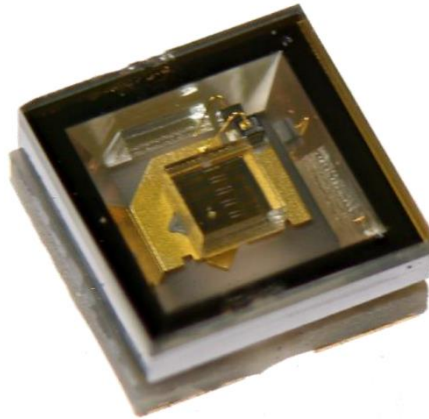
Ceramic SMD Ultraviolet LED with Flat Top
