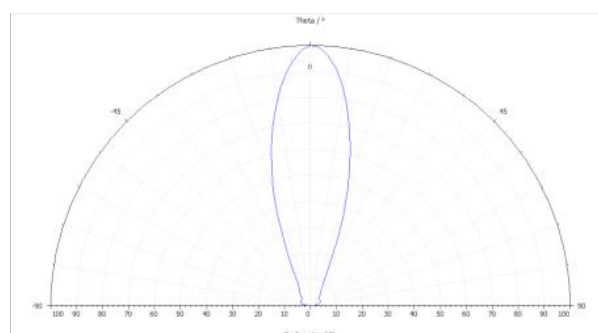
Radiation Pattern
