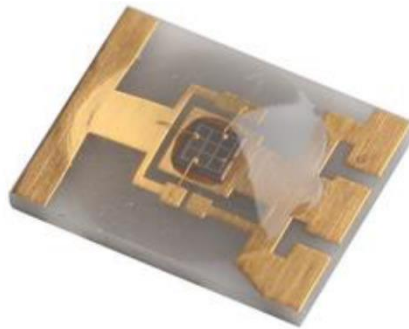
High Power Deep blue LED with Glob Top
