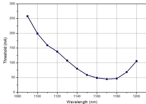
Threshold current
