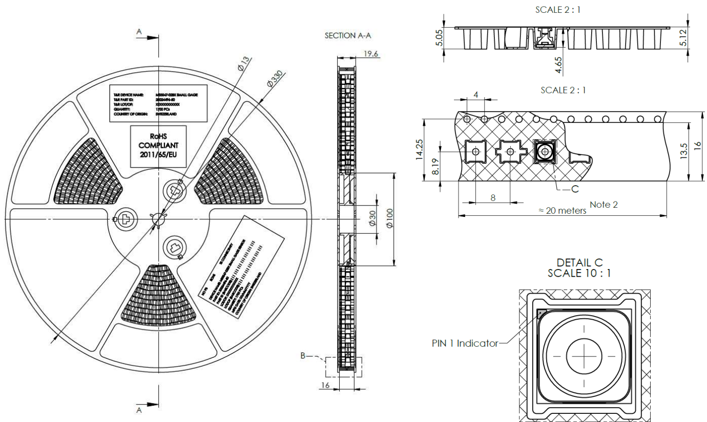
Figure 50: Shipping package.
