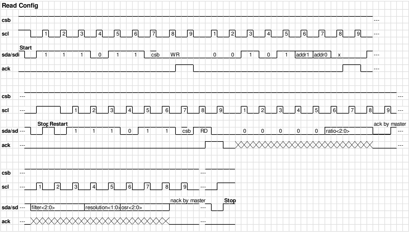
Figure 40: Read Config.
