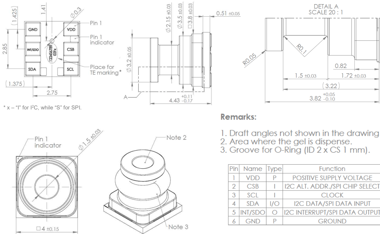
Figure 48: Package outline and pin configuration.
