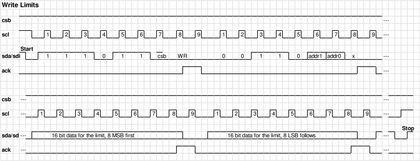
Figure 41: Write Limits.
