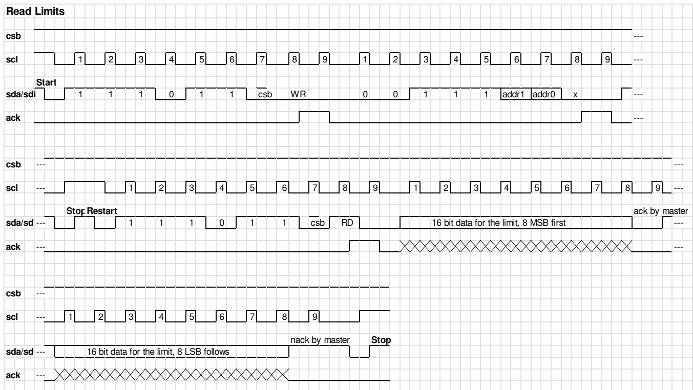
Figure 42: Read Limits.
