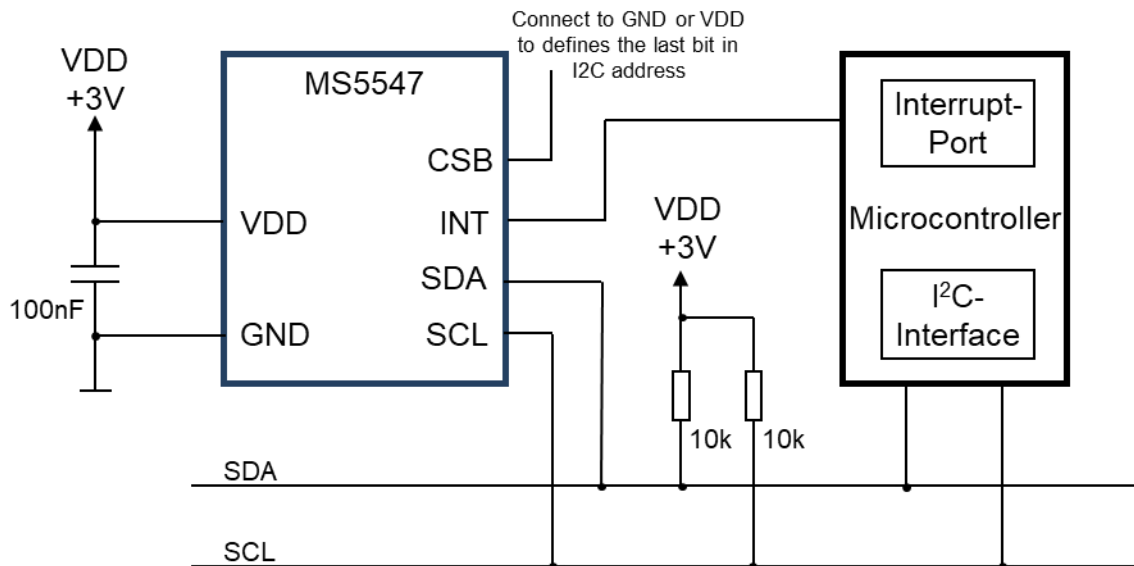
Figure 30: Typical I 2 C application circuit.
