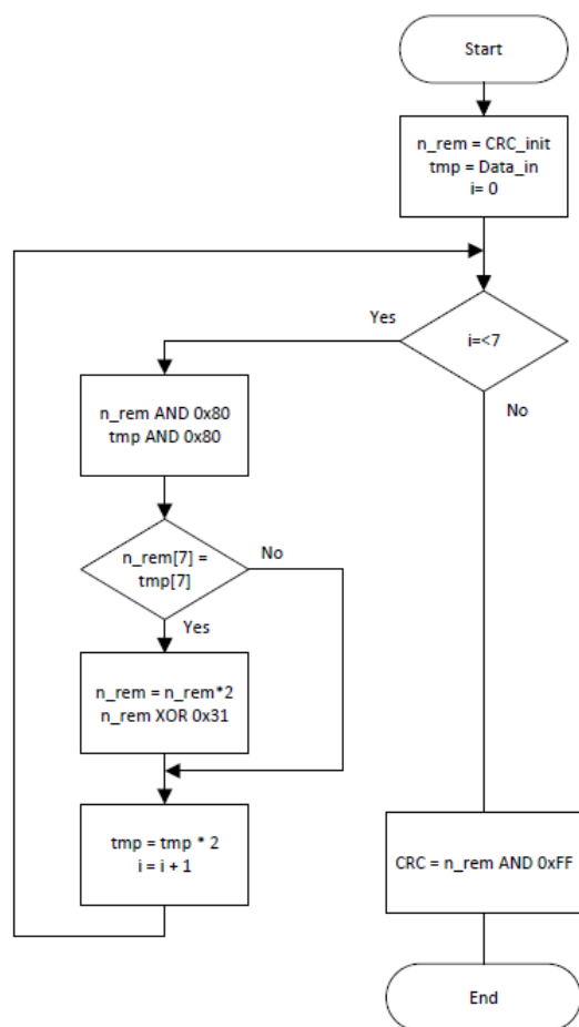
Figure 47: CRC8 calculation flowchart &amp; Excel Calculation function.
