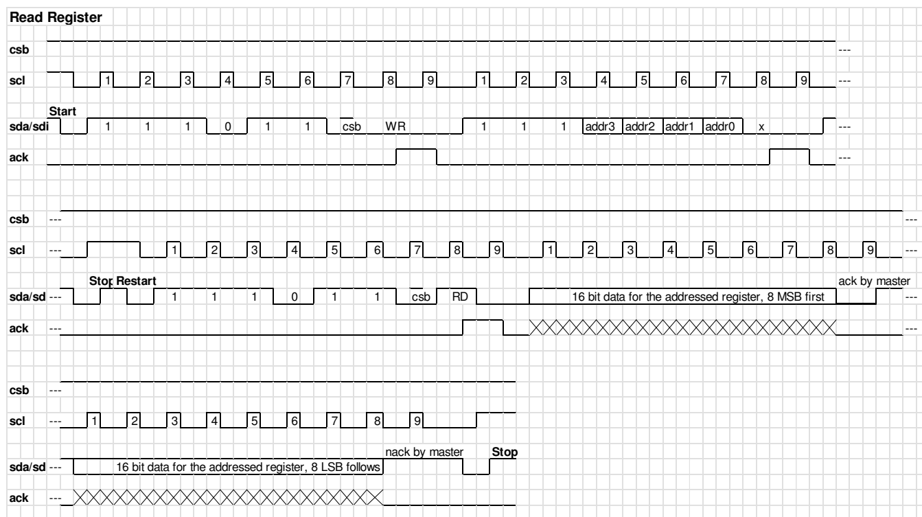
Figure 45: Read Register.
