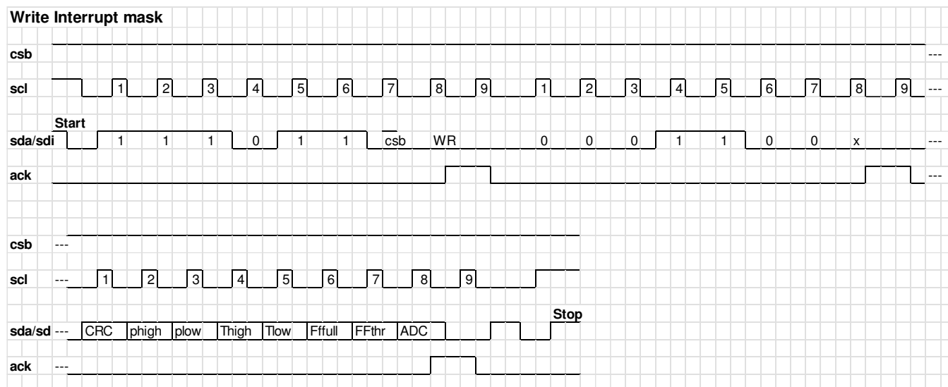
Figure 35: Write Interrupt mask.
