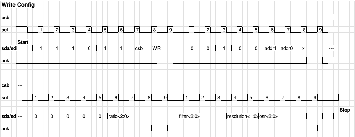
Figure 39: Write Config.
