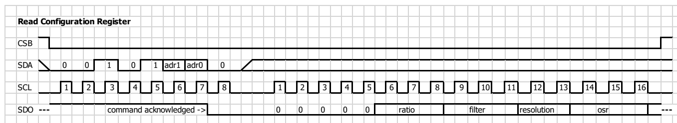
Figure 18: Read Config in SPI mode 0.
