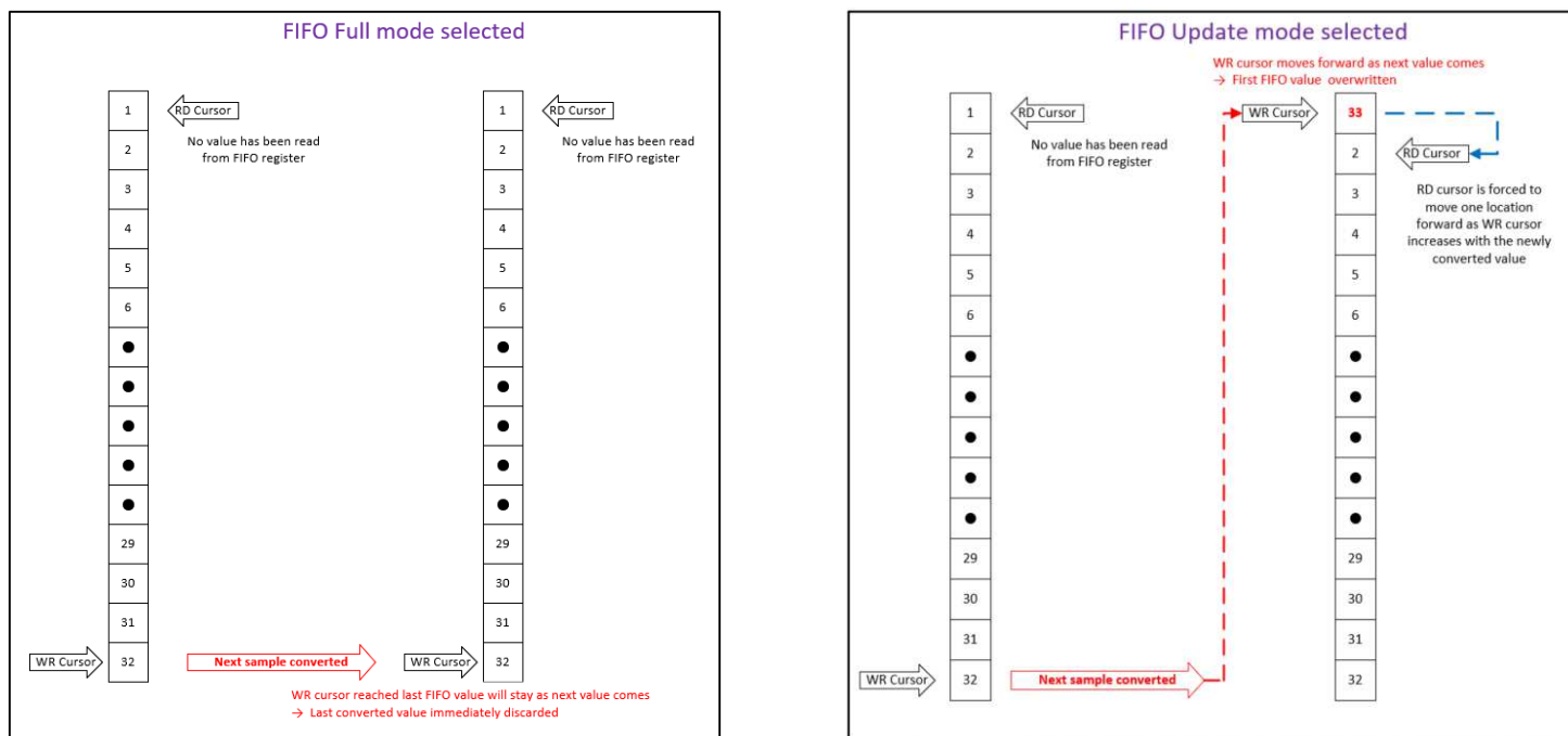
Figure 1: FIFO Modes.
