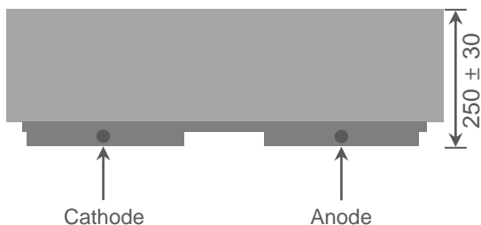
Cross Section
