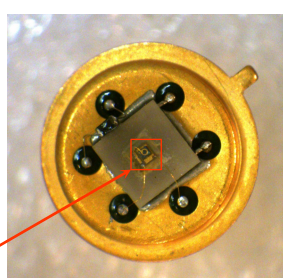
LED chip
