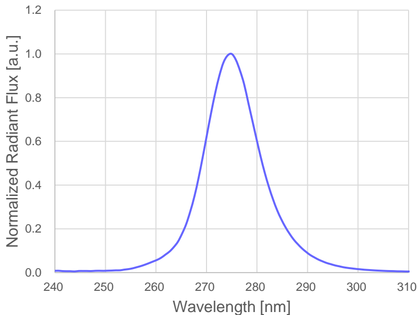
< Spectrum, I_F = 20\text{ mA} >
